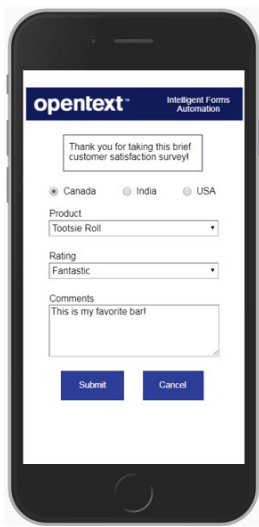
Mobile forms
