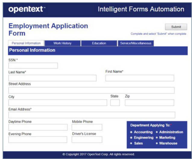
Tabbed forms
