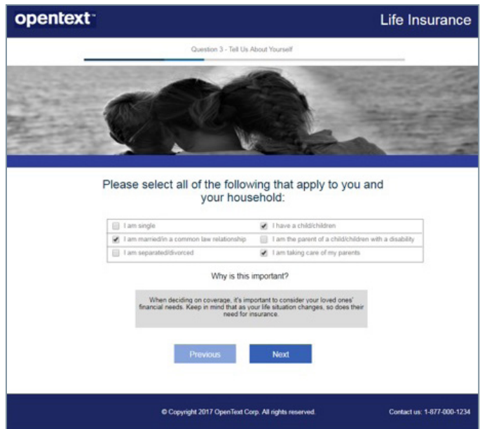
Wizard forms
