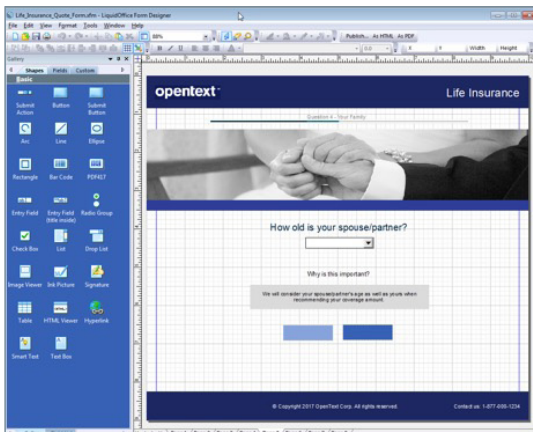
Forms Designer
